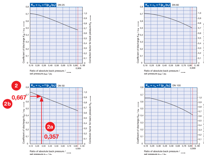
Diagram for evaluation of the coefficient of discharge ( K_{dr}/\alpha_w ) or K_b in reference with the ratio of absolute back pressure / set pressure ( p_{a0}/p_0 )
